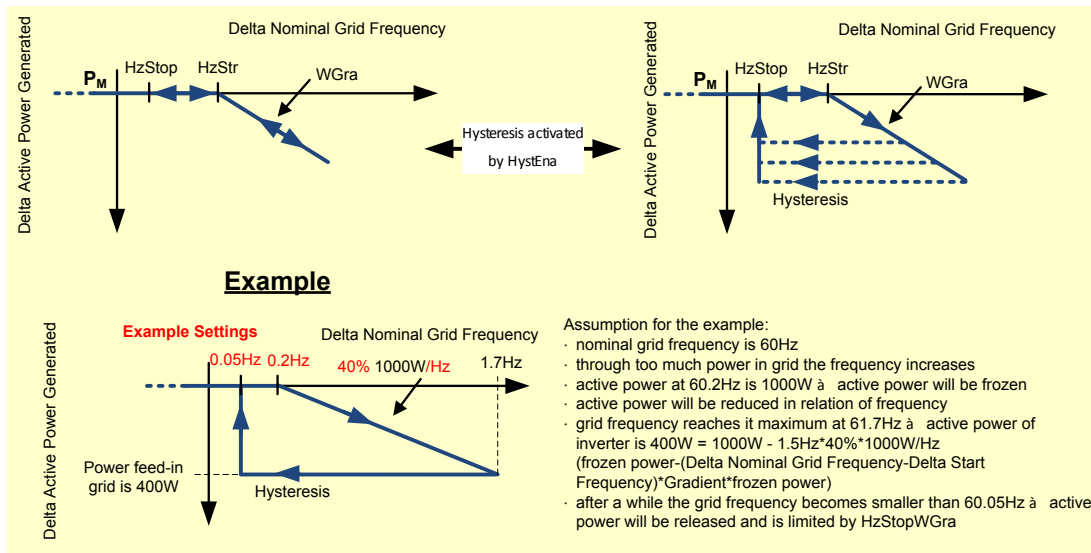
Figure 9: Parameter-Based Frequency-Watt Control
