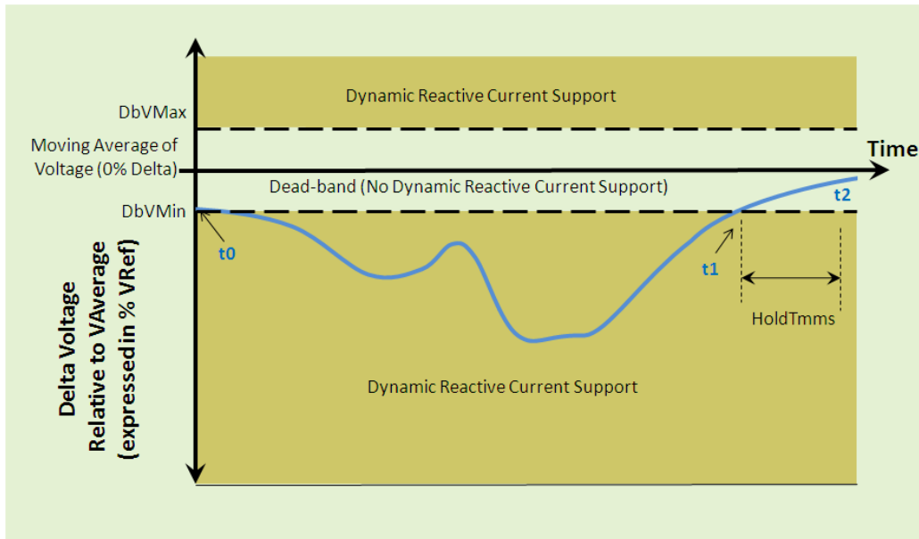
Figure 12: Activation Zones for Reactive Current Support
