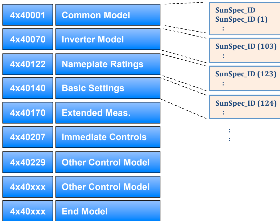
Figure 1: Chained Inverter Control Models
