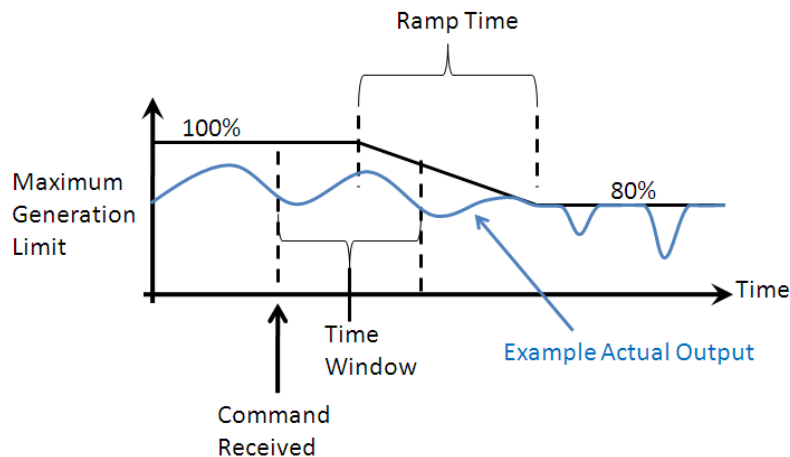
Figure 2: Example Time Window and Ramp Time
