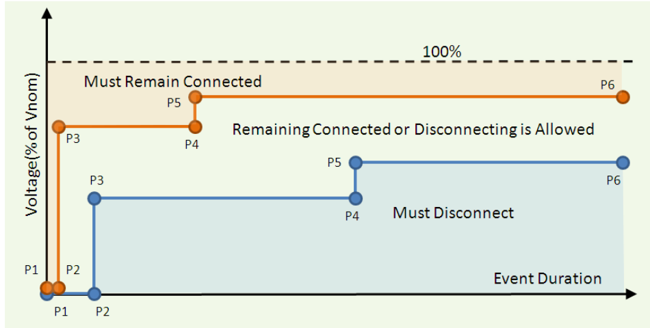
Figure 13: Use of Curves to Define LVRT Area
