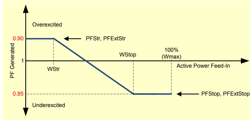
Figure 15: Example Watt-PF Curve
