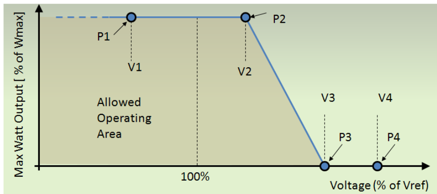
Figure 16: Example Voltage-Watt Curve
