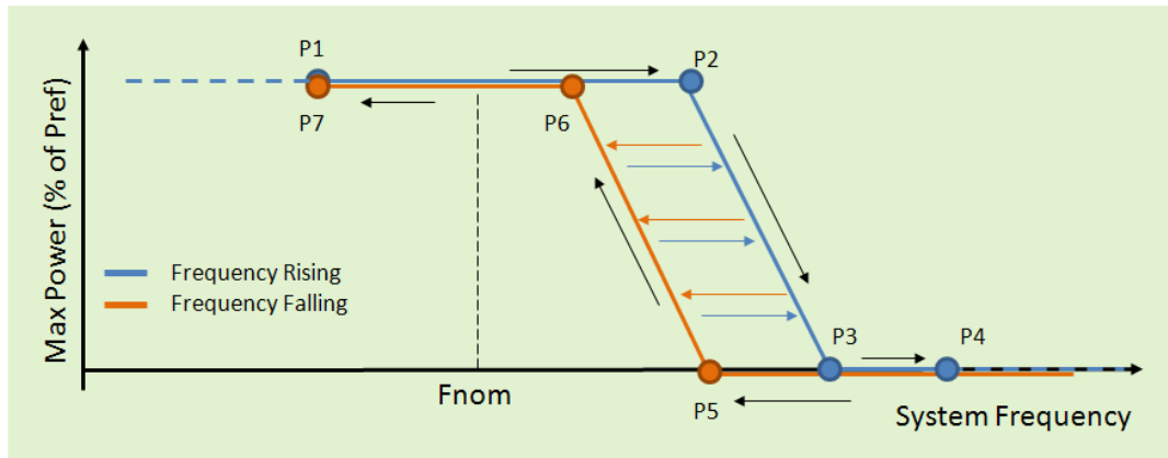
Figure 10: Curve-Based Frequency-Watt Control with Hysteresis
