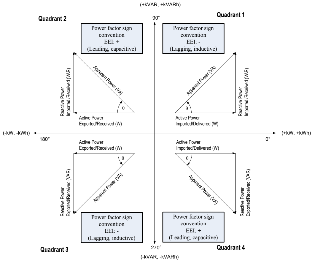
Figure 6: EEI Power Factor sign convention
