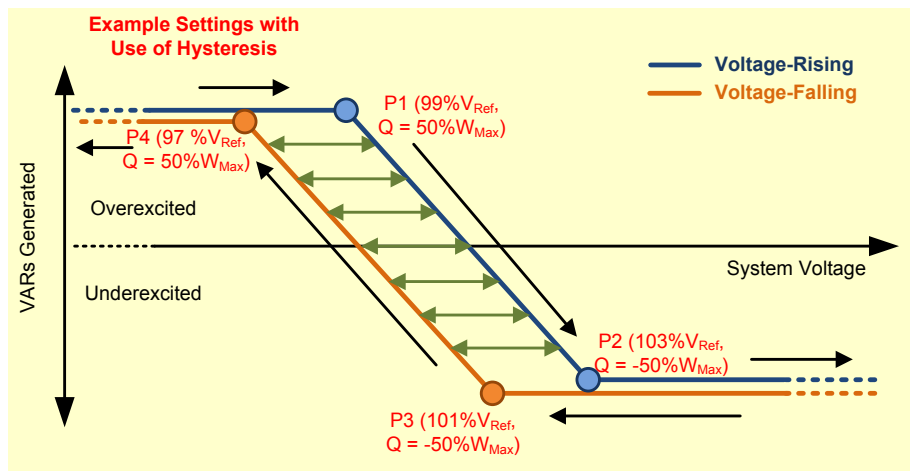
Figure 7: Volt-VAR Array Setting with Hysteresis
