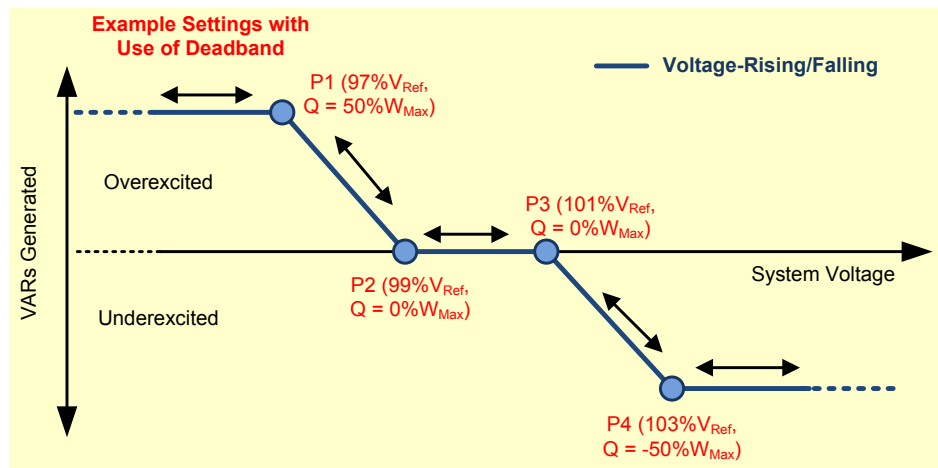
Figure 8: Volt-VAR Array Setting with Deadband
