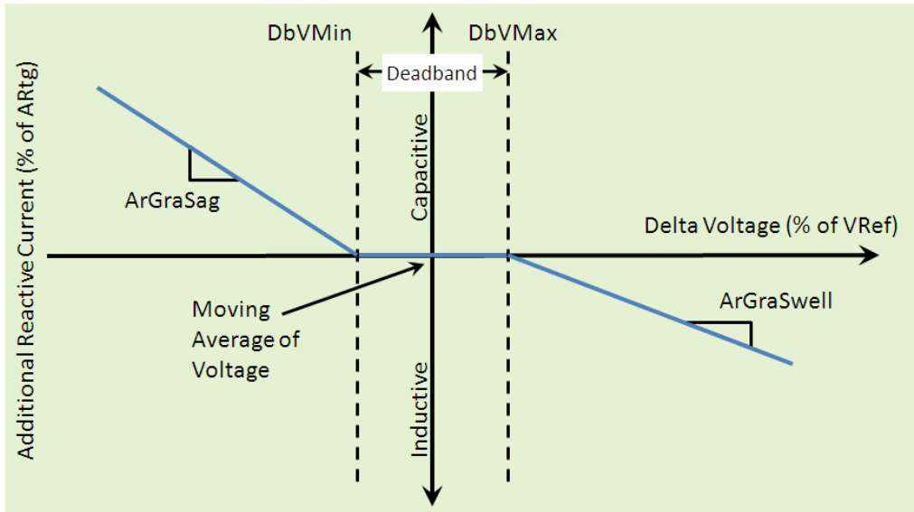
Figure 11: Dynamic Reactive Current Support
