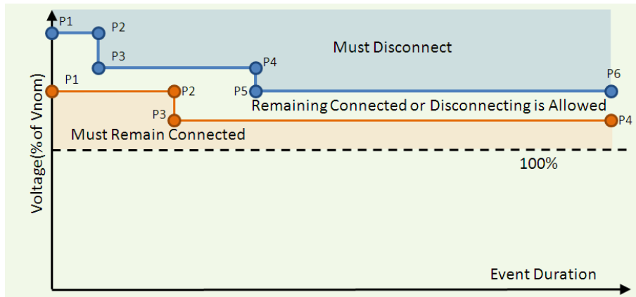
Figure 14: Use of Curves to Define HVRT Area
