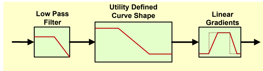
Figure 3: Transfer Function for Curve-Based Controls
