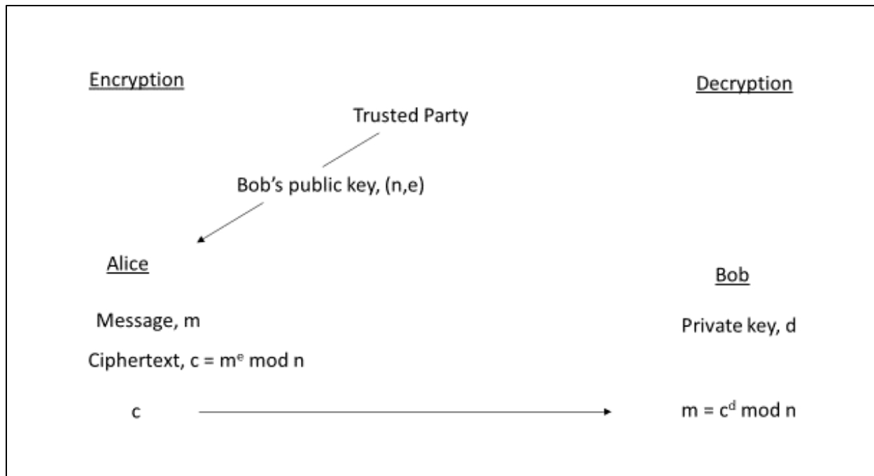
Figure 13: RSA Encryption/Decryption.
