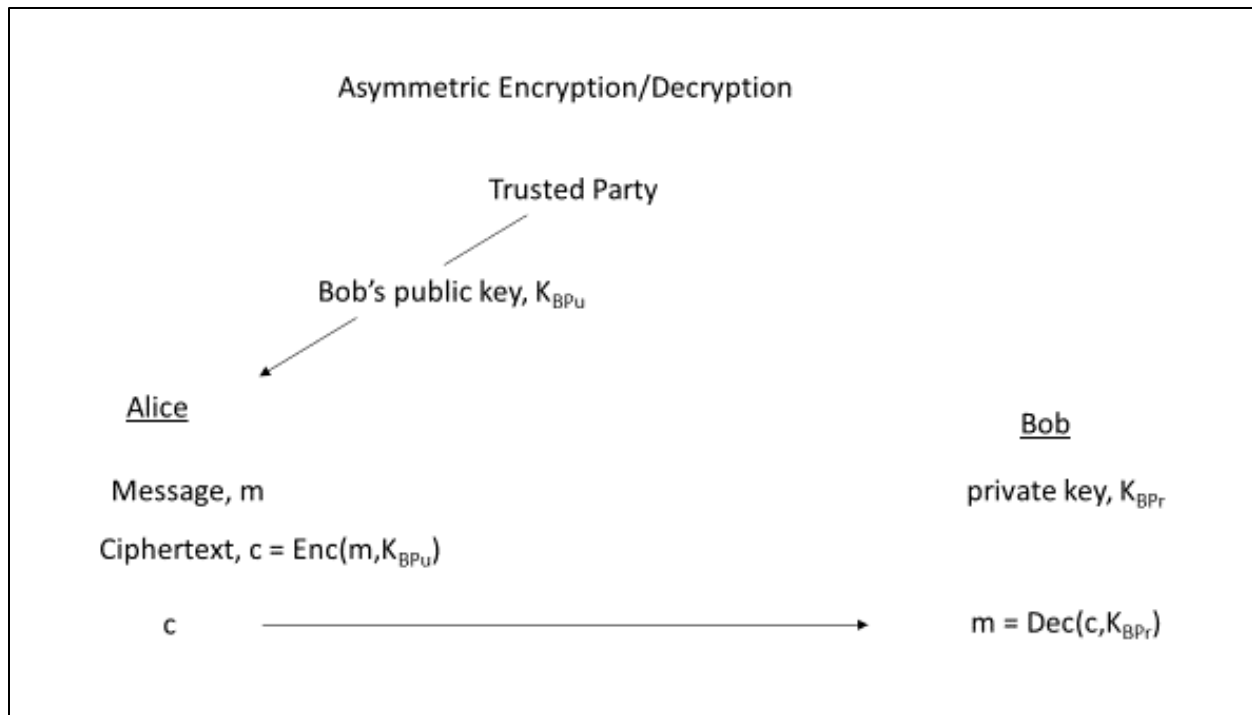
Figure 12: Asymmetric Encryption/Decryption.
