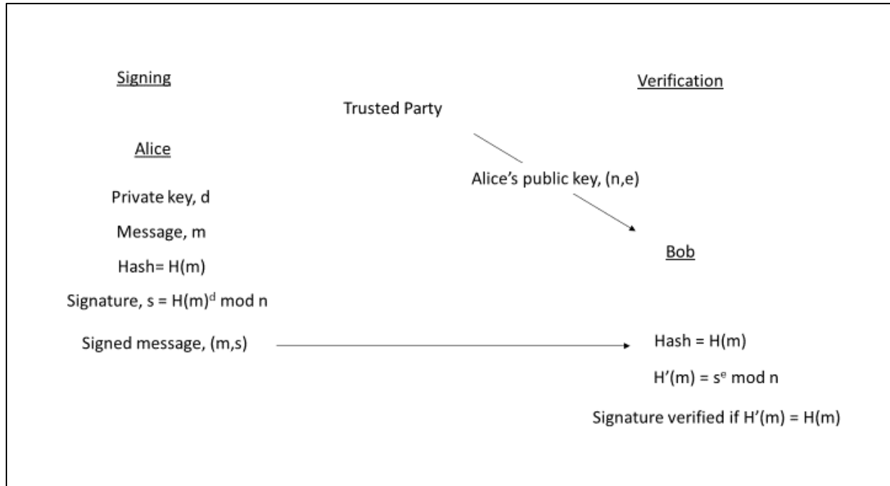
Figure 17: RSA Signature/Verification.
