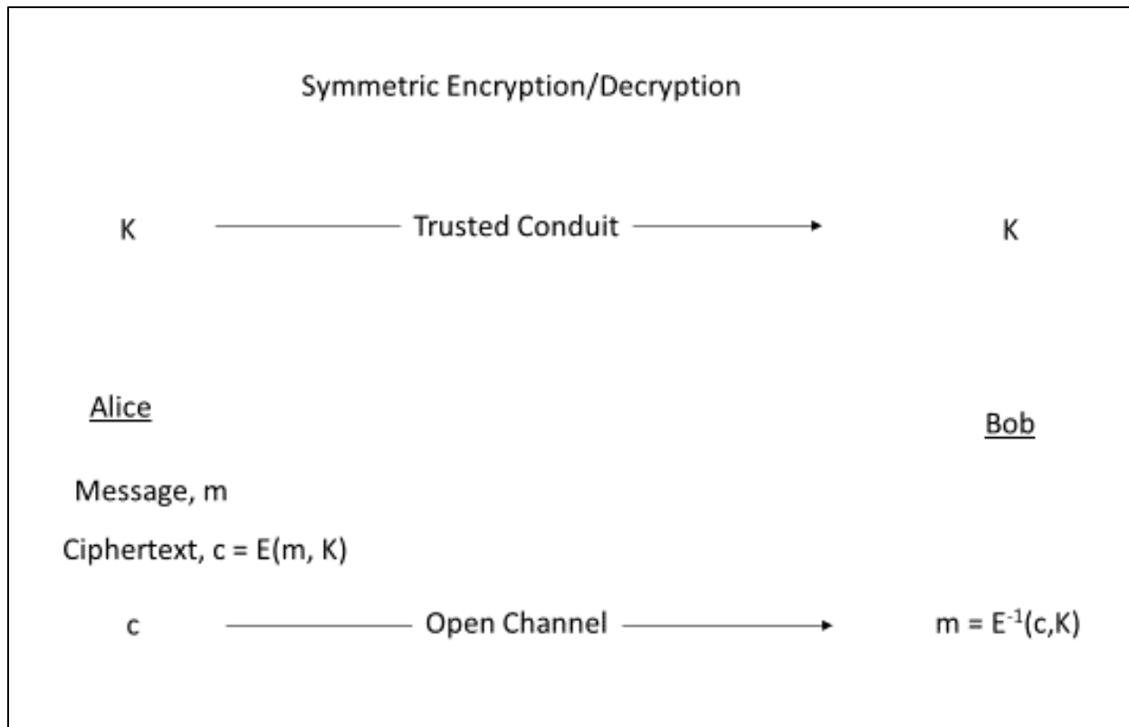
Figure 11: Symmetric Encryption/Decryption.
