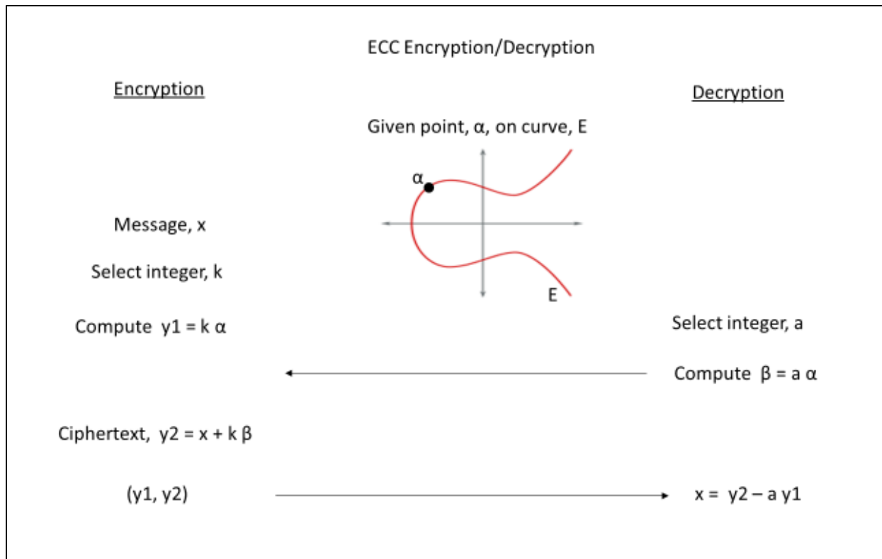
Figure 15: ECC Encryption/Decryption.
