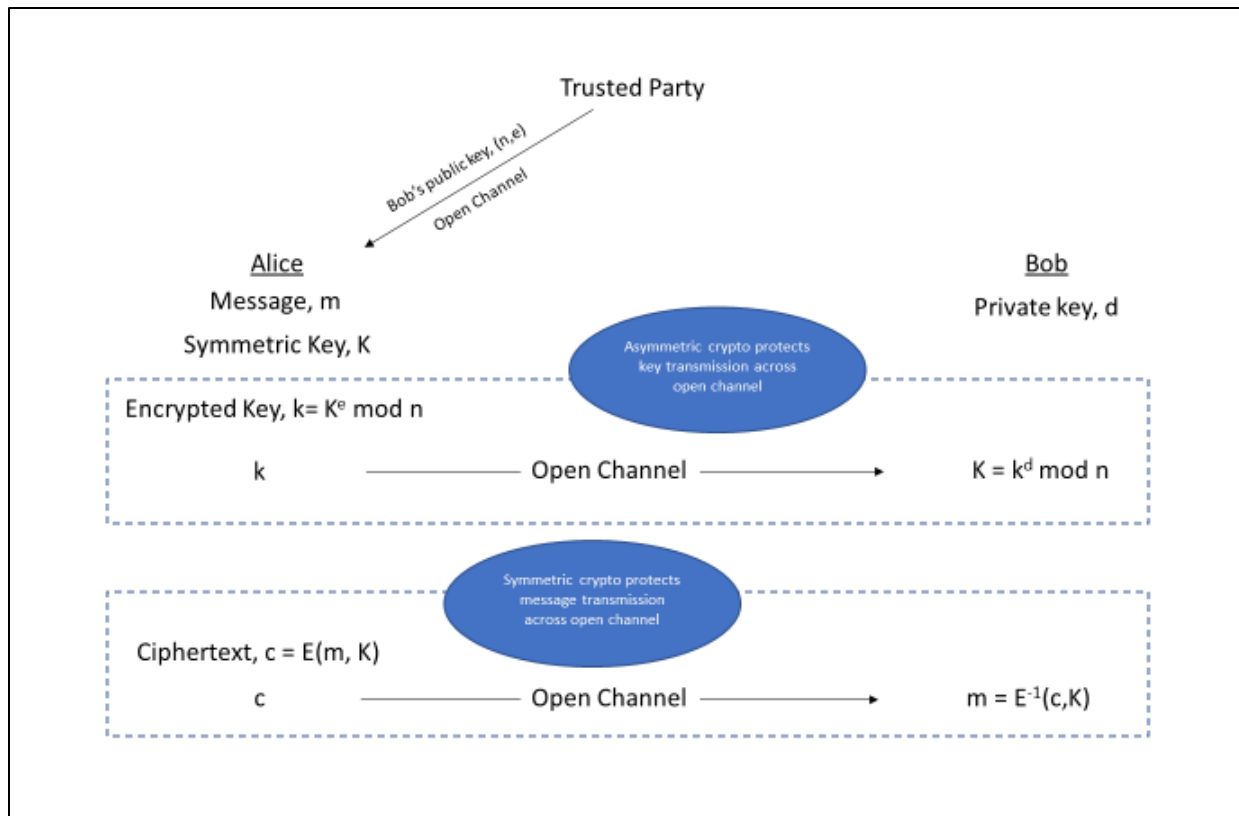
Figure 16: Asymmetric Crypto Enables Symmetric.
