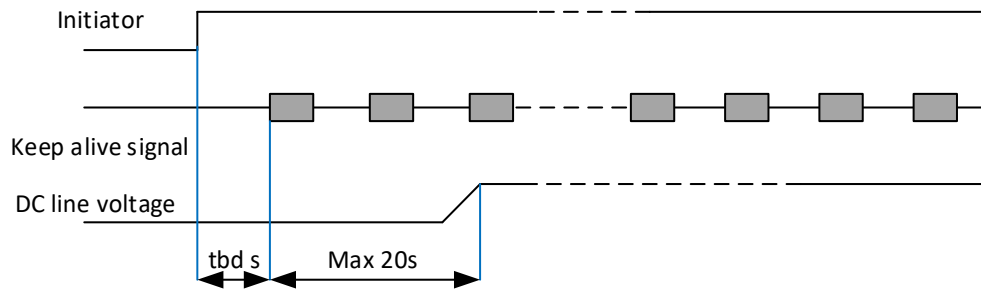
Figure 5.1: Start Process interoperability test timing
