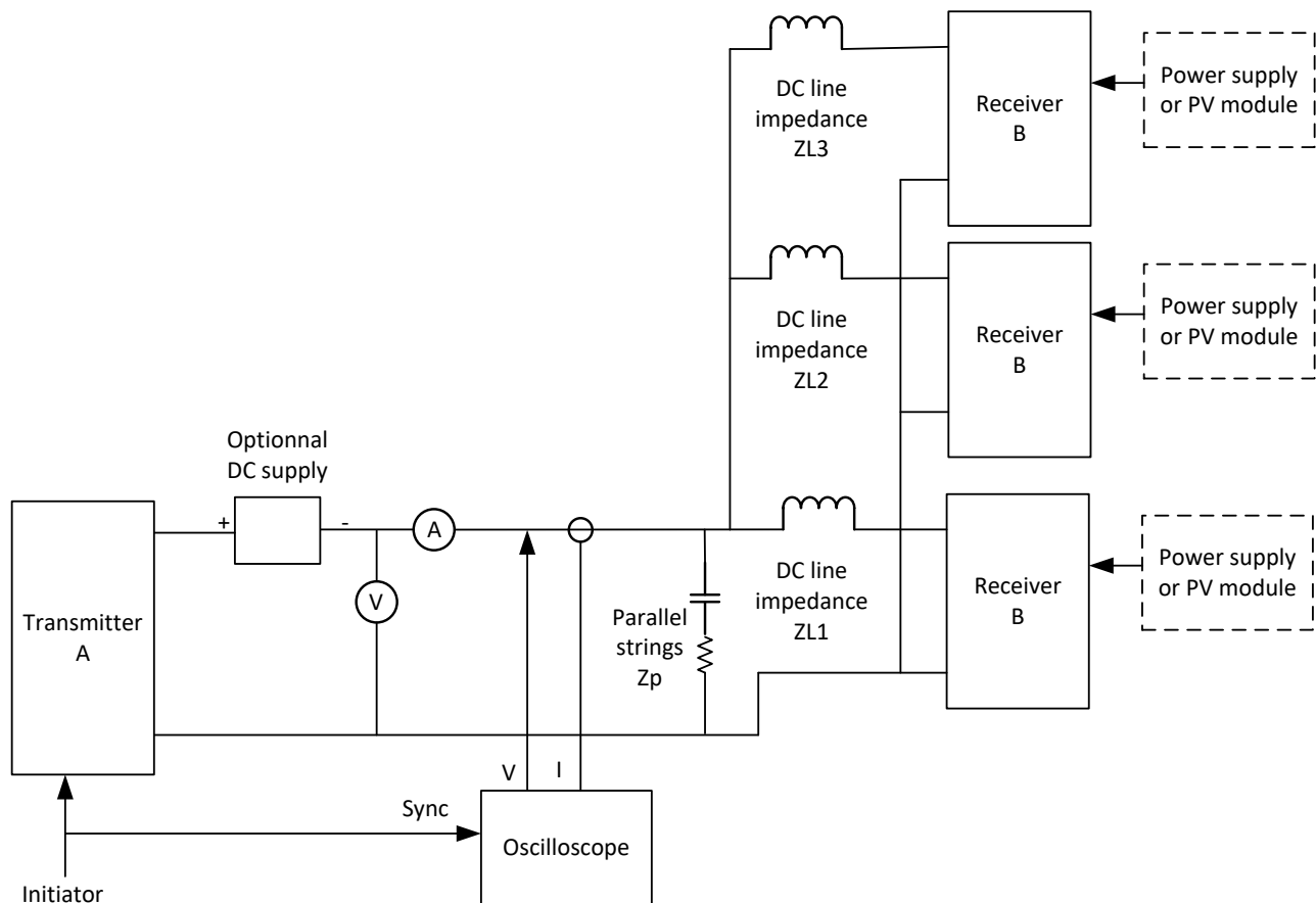
Figure 5.4: Multiple Receiver interoperability test diagram
